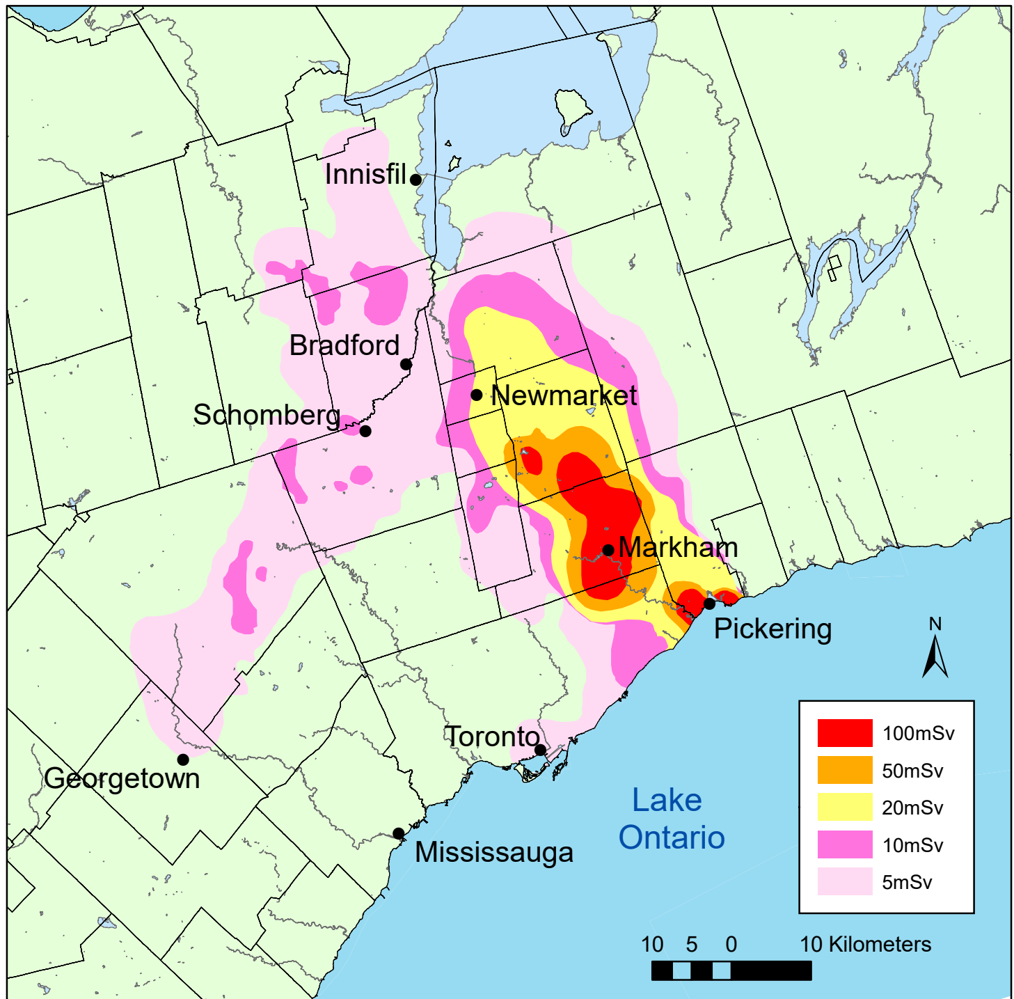
Figure 2: High Doses (red, orange and yellow areas) Fukushima Fallout Centred on Pickering NGS Superimposed on Toronto and Surrounding Areas
