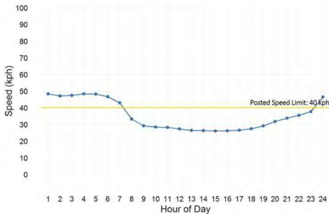
Figure 14. Vancouver 24 Hour Speed Profiles
