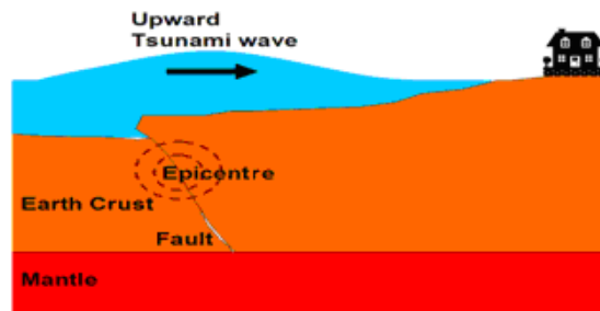
Figure 5.1 Generation of a Tsunami
