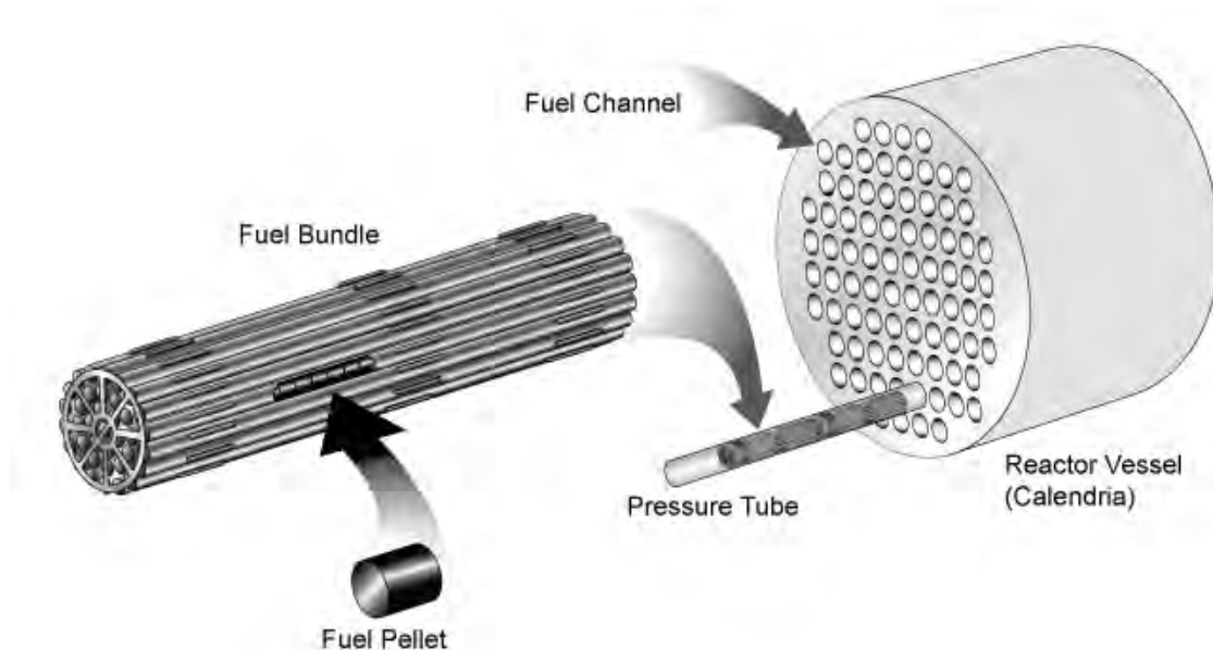
Figure A.1 Arrangement of Fuel Bundles in a CANDU Calandria
