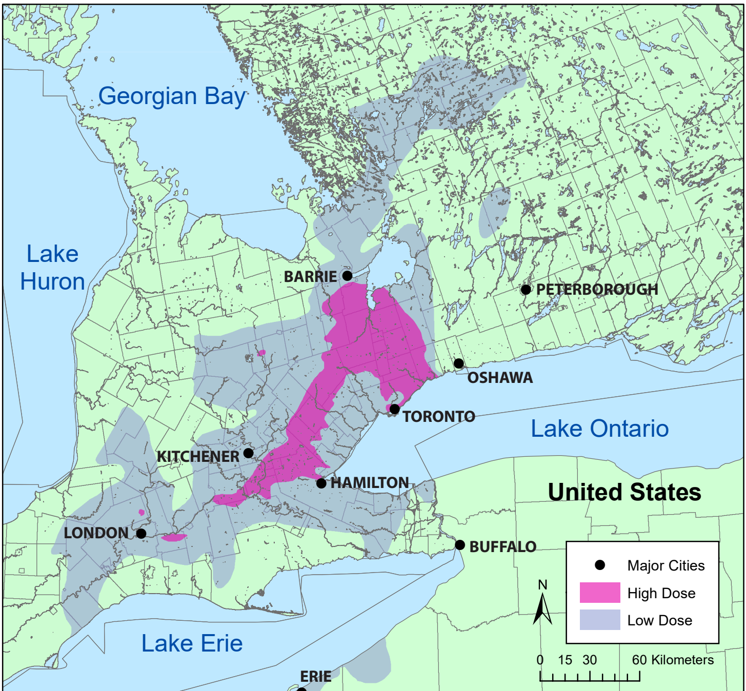
Figure 1: Low Doses (light blue area) Fukushima Fallout Centred on Pickering Superimposed on Southern Ontario
