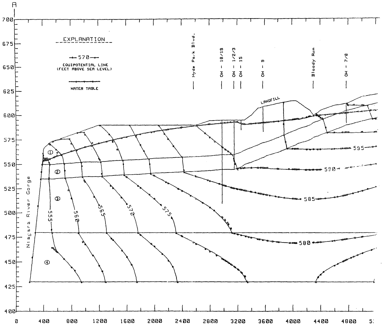
CROSS - SECTIONAL DISTANCE FROM NIAGARA RIVER Figure 5. -- Simulated water table position and head
