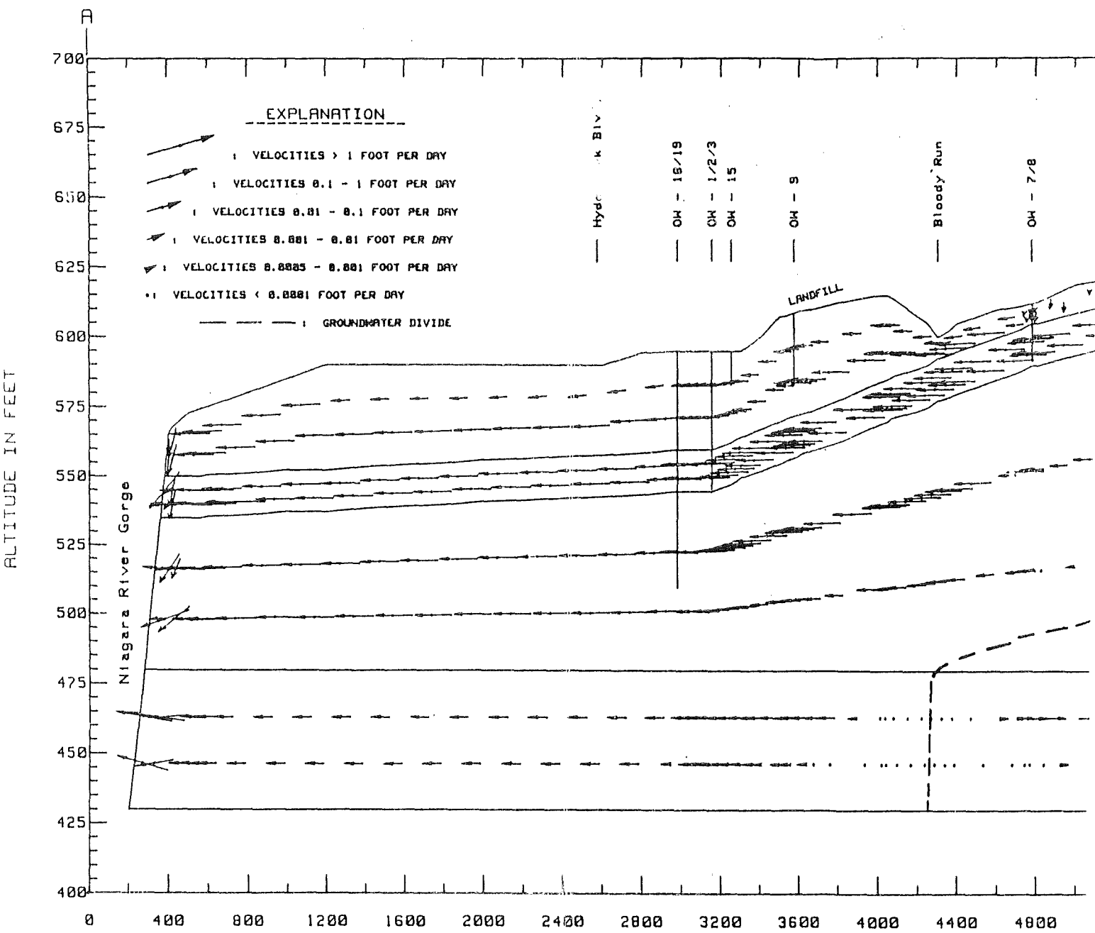
Figure 6. -- Elemental Darcy Velocity
