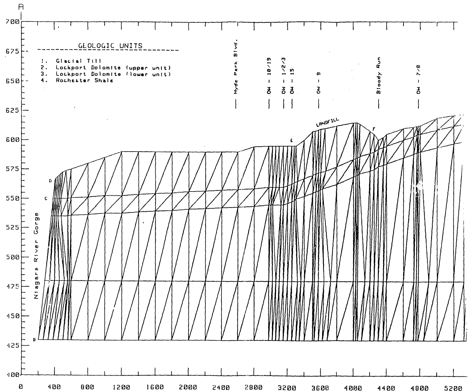
Figure 4. -- Finite element idealization
