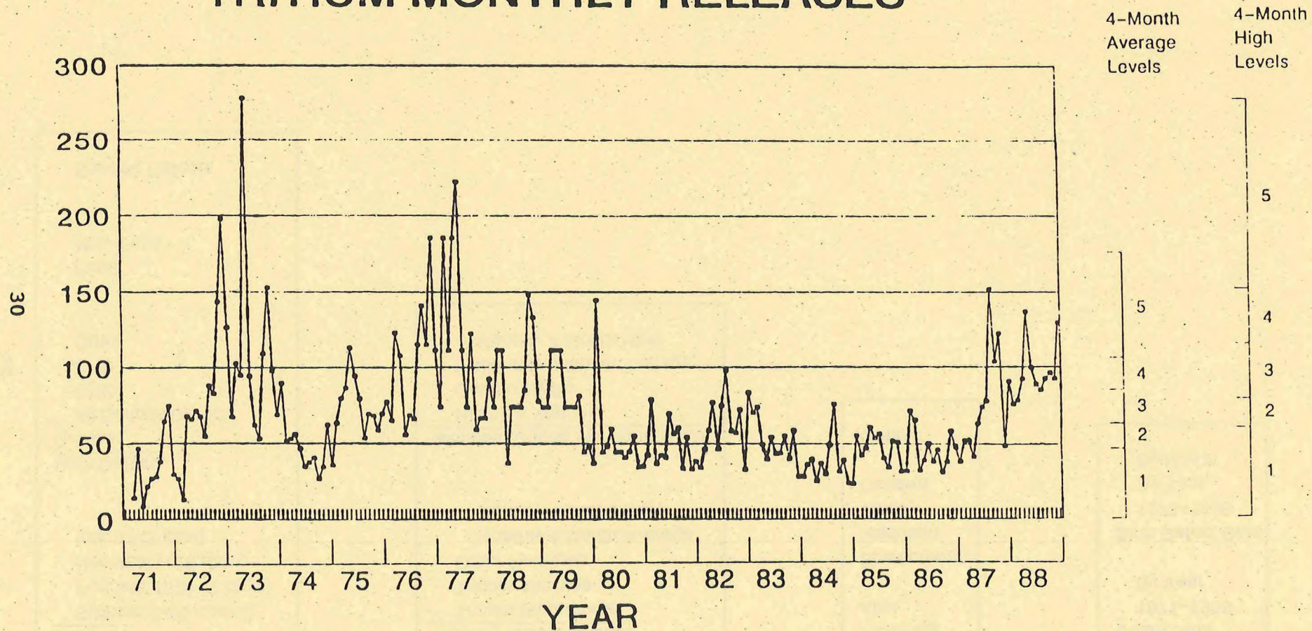
Figure 2. PICKERING NGS TRITIUM MONTHLY RELEASES
