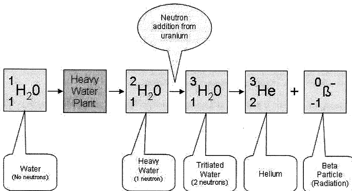
Diagram 1: Tritiated Water Decay
