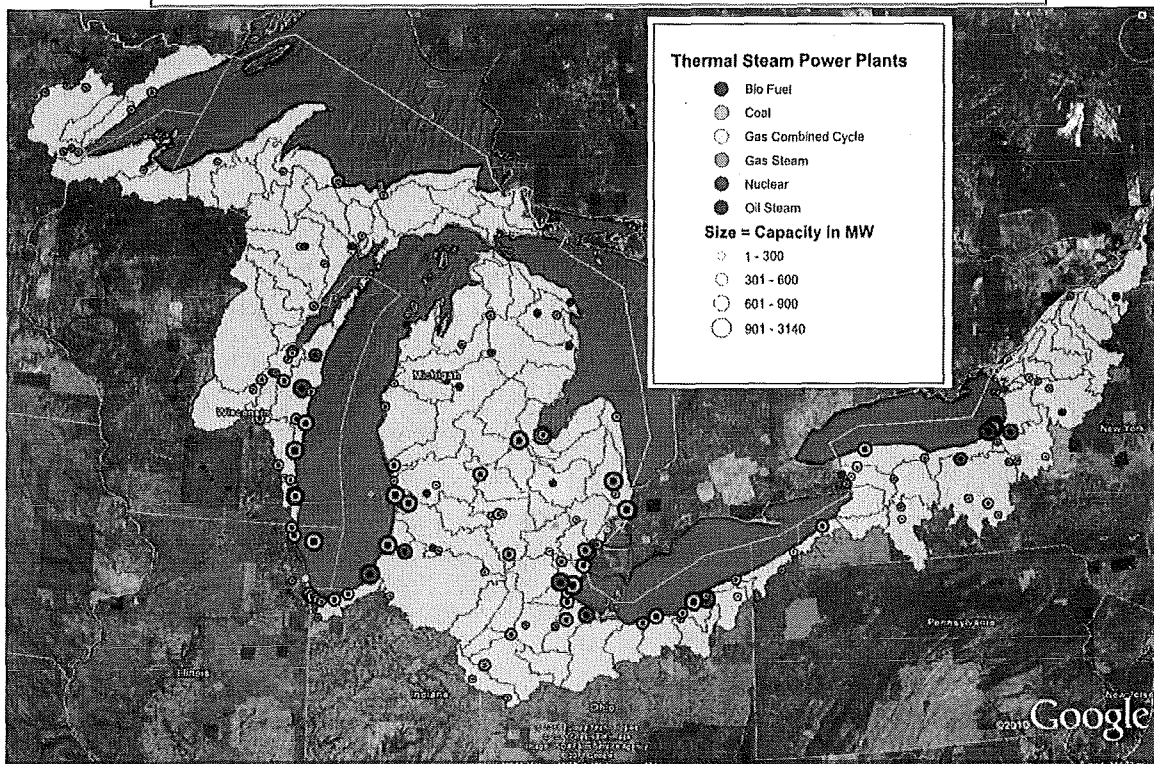
Figure 7: Electric power generation capacity by state and water use sector in 2007 (top) and location of the thermoelectric power plants in the basin (below). Only those plants physically located within the Great Lakes watershed are included.
