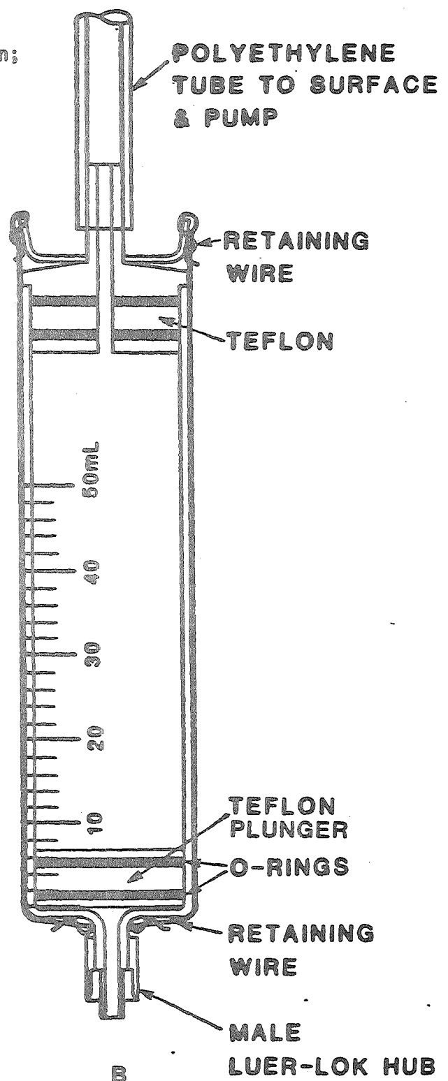
Figure 2. Down-hole cartridge sampling device including:
